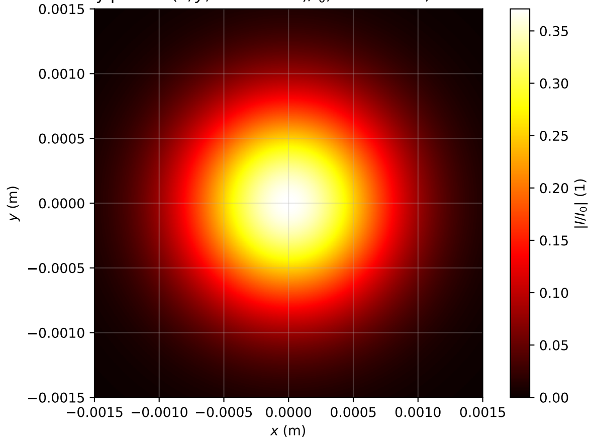
Intensity profile I(x, y, z = 2.786m)/I_0 , P_{in}=0.1P_{cr} , artificial time
